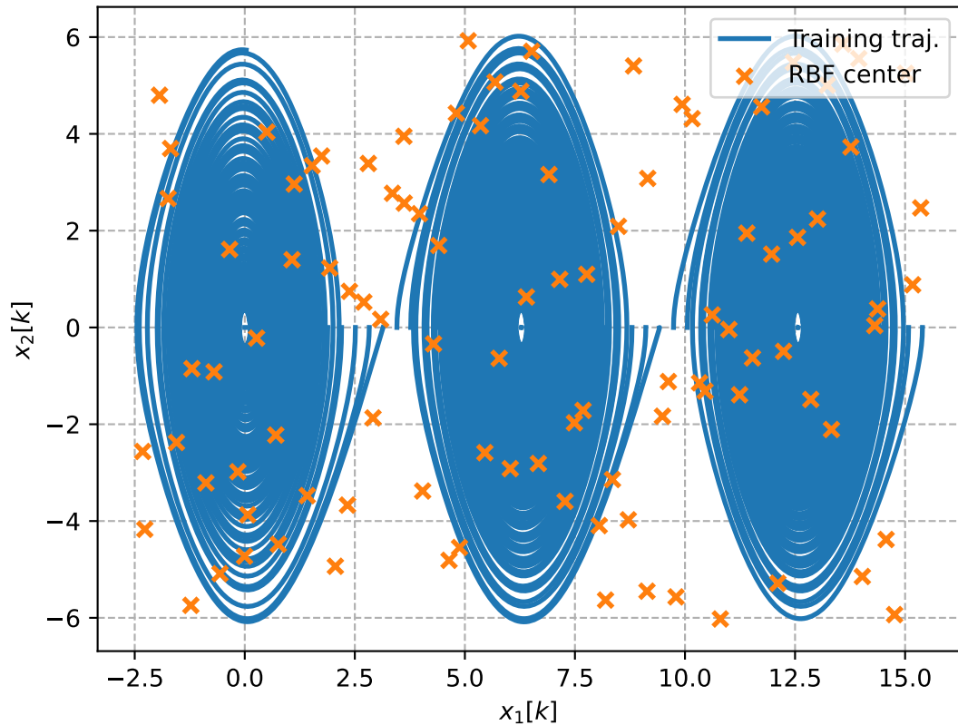
Training trajectories and RBF centers
