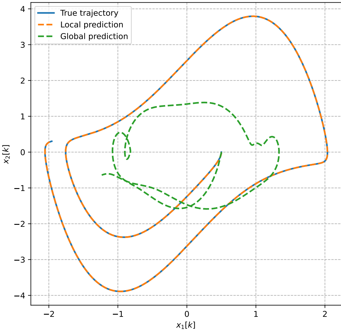
True and predicted phase-space trajectories
