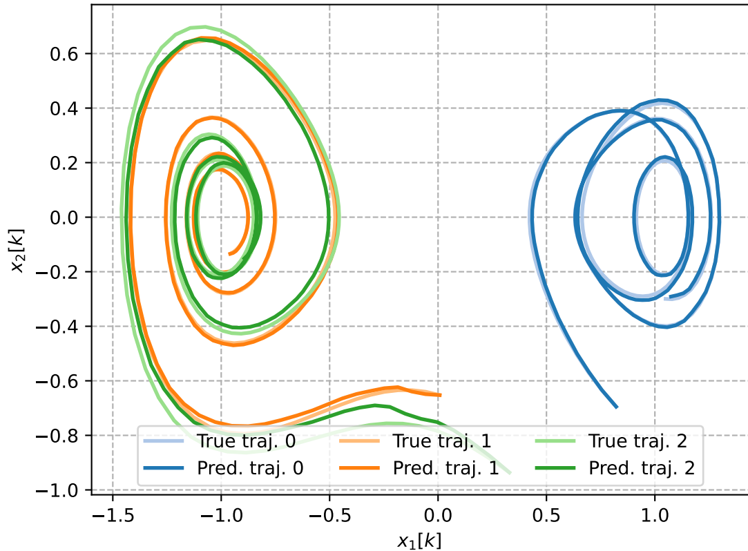
Randomly binned features: true and predicted trajectories
