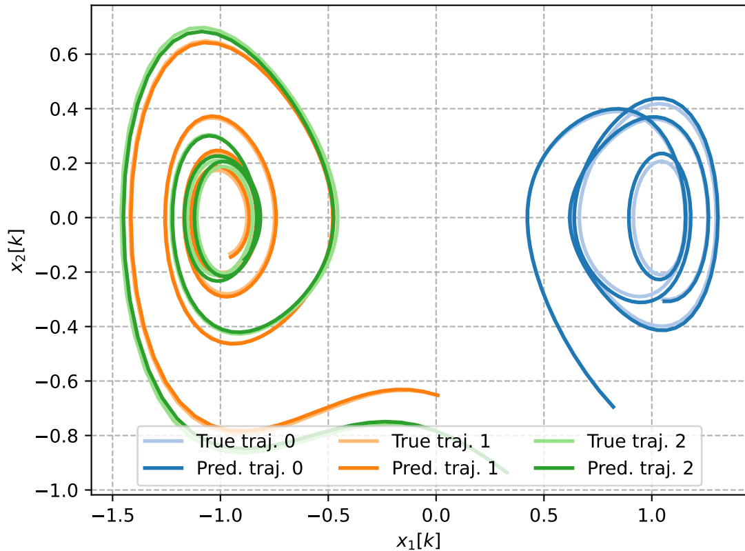
Random Fourier features: true and predicted trajectories
