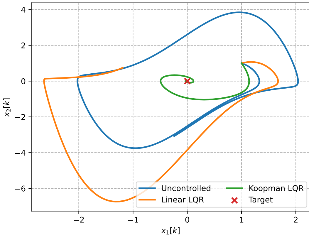
Comparison of linear and Koopman LQR controllers
